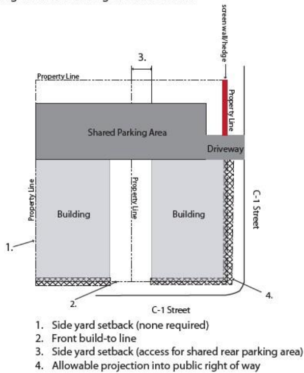
Figure 13.1 Building Site Placement
