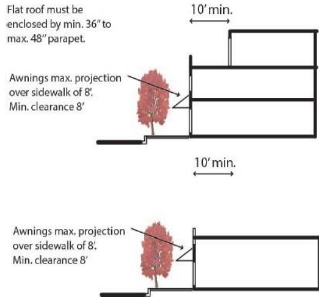
Figure 13.2 3rd Story Setback Illustration
